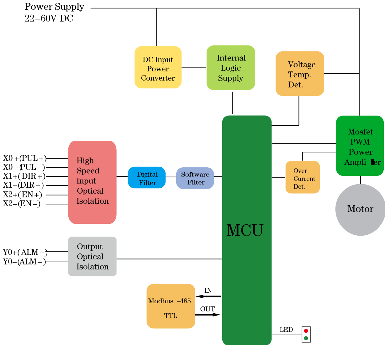
MD57HS-ICE-R Block Diagram
